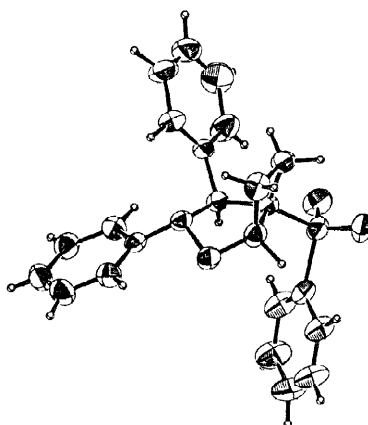
Figure 1 : ORTEP drawing of 1d
